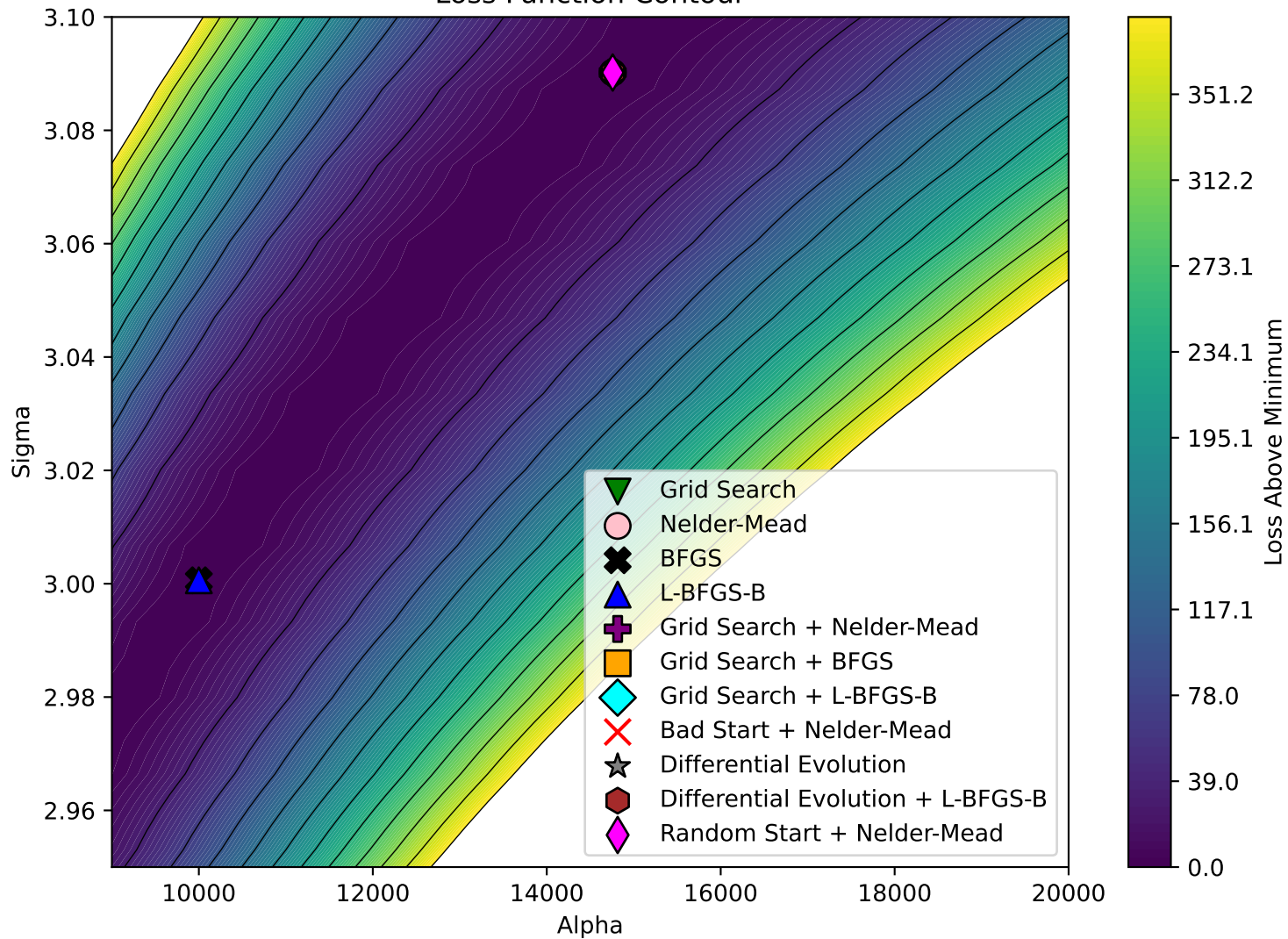
Loss Function Contour
